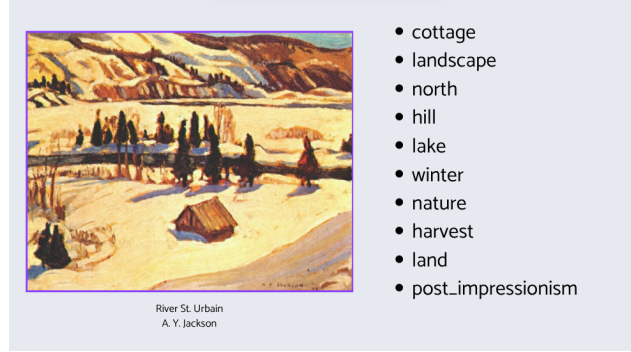
Figure 6: Example of concepts extracted using CLIP
