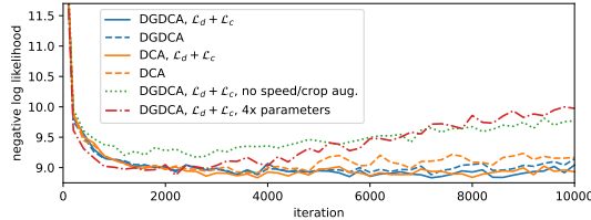
Figure 2: Validation negative log likelihood over training.
