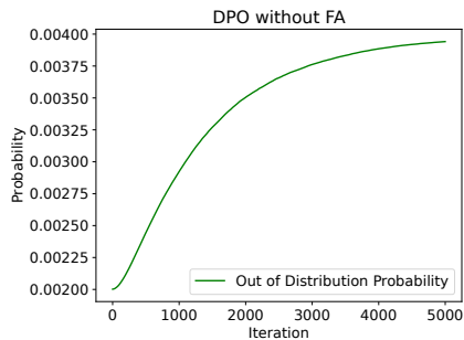
Figure 3: Extrapolation behavior of DPO without function approximation. We plot the average probability of out-of-distribution responses along the training and DPO assigns increasing probability to out-of-distribution responses.
