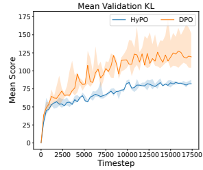
Figure 1: Mean validation reverse KL to the reference policy when DPO and HyPO are trained for 5 epoch on the TL;DR dataset. We repeat the experiment for 3 random seeds and plot the median and the shaded areas denote the min and max over the 3 repetitions.
