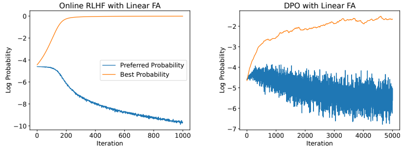
Figure 2: Extrapolation behavior of Online RL method and DPO under linear function approximation. We plot the mean log probability of the preferred responses and the log probability of the best response, which is unseen in the training data. We see that both algorithms correctly assigns increasing probability to the best response.
