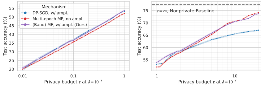
Figure 12: Our banded matrices consistently perform at least as well as the best prior method in each range of \epsilon . Around \epsilon \approx 1 , we observe significant utility benefits from the banded mechanism around 2 – 3 percentage points over DP-SGD. We only optimize the Band MF over \hat{b} \in [0, n/k] which leads to a regime around \epsilon > 5 where the it performs worse than the Multi-epoch MF of Choquette-Choo et al. [15]; \hat{b} = n is equivalent to this approach modulo the sensitivity definition which we exclude to emphasize the regime we improve on. Empirical setup is in App. H.
