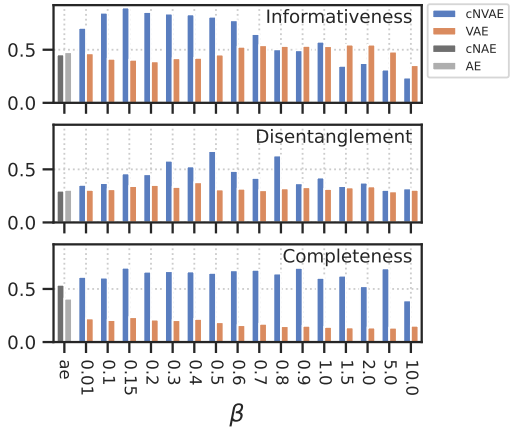
Figure 5: Evaluating the learned latent codes using the DCI framework [22]. Larger values are better for all metrics. Note that informativeness is closely related to untangling [20, 21]. See also Fig. 9.
