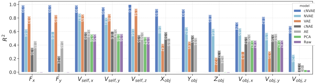
Figure 4: Hierarchical VAE untangles underlying factors of variation in data. The linear decodability of ground truth factors (x-axis) from different latent codes is shown. Untangling scores averaged across all ground truth factors are cNVAE = 0.898, NVAE = 0.639, VAE = 0.548, cNAE = 0.456, AE = 0.477, PCA = 0.236, and Raw = 0.235. For variational models, the best performing \beta values were selected: cNVAE, \beta = 0.15 ; VAE, \beta = 1.5 (see Supplementary section 9.5 for more details).
