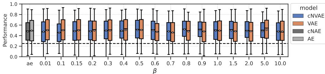
Figure 7: All models (pretrained on fixate-1 ) perform comparably in predicting MT neuron responses. Dashed line corresponds to the previous state-of-the-art on this data [106].
