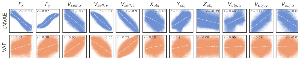
Figure 11: For each ground truth factor and model, we identified a single latent variable that displayed the highest (Pearson) correlation with that variable. The ground truth factors exhibited greater linearity within the latent space of cNVAE compared to VAE. Scatter points correspond to data samples from the test set. x-axis, the value of ground truth factors; y-axis, the value of latent variables.
