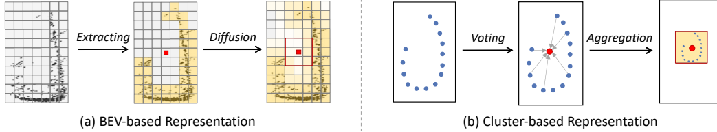
Figure 1: Illustration of (a) context-aware BEV-based representation[10] and (b) object-centric cluster-based representation. The BEV representation can capture the rich contextual information of an object. However, the missing feature of the center point (red square), which is also the key to making the prediction, is diffused from occupied voxels. The cluster-based representation is generated using the voting mechanism by aggregating the foreground points into the object-specific feature for the voting center (red dot). This representation mainly focuses on the foreground points and fails to utilize the contextual information.
