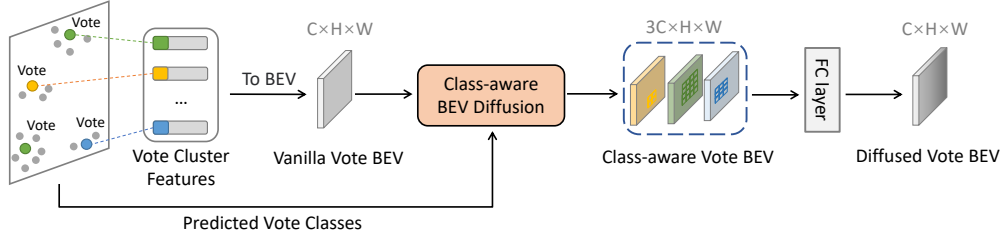
Figure 3: Illustration of Cluster Feature Diffusion (CFD) module. We first transform the vote cluster features to the BEV space based on the position of each vote, forming a sparse representation termed vanilla vote BEV features. Next, the non-empty grids of vanilla vote BEV are adaptively expanded to their neighboring regions according to the predicted class of the vote through a class-aware BEV diffusion block. Finally, we use a fully connected layer to project the class-aware vote BEV to the same channel dimension as the vanilla vote BEV, thus obtaining a diffused vote BEV feature.
