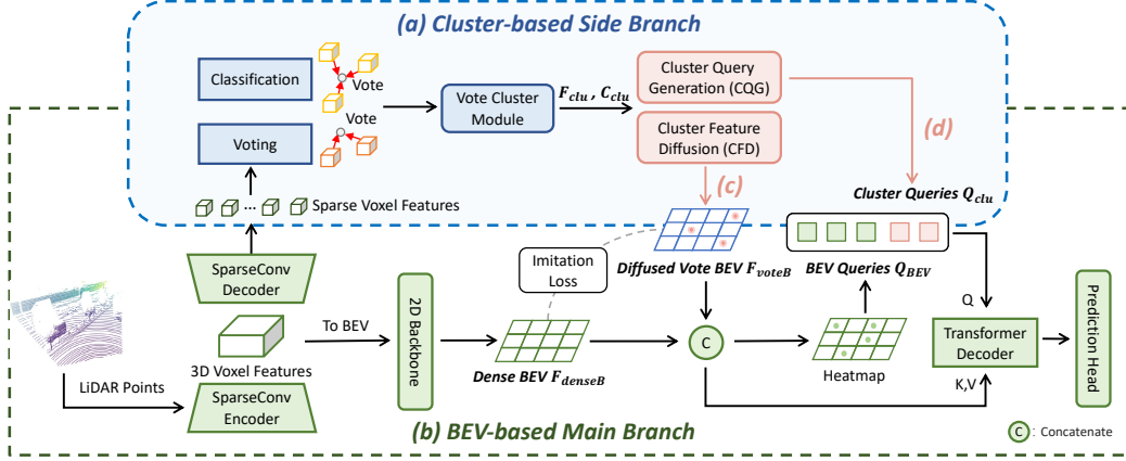
Figure 2: The overall framework of CluB. The cluster-based side branch (a) is integrated into the BEV-based main branch (b) through a two-step scheme, i.e. , feature-level integration (c) and query-level expansion (d). Specifically, the raw point clouds are first voxelized and then fed into the sparse U-Net to extract both 3D voxel features and sparse voxel features. The former is used to obtain the dense BEV feature. The latter is processed in the cluster branch to generate a set of vote cluster features \mathbf{F}_{clu} and corresponding voting centers \mathbf{C}_{clu} . Based on the two outputs, i.e. , \mathbf{F}_{clu} and \mathbf{C}_{clu} , the Cluster Feature Diffusion (CFD) module obtains a diffused vote BEV feature \mathbf{F}_{voteB} to enhance the dense BEV feature \mathbf{F}_{denseB} supervised by an imitation loss, and the Cluster Query Generation (CQG) module outputs a set of top-ranking cluster queries \mathbf{Q}_{clu} , which are concatenated to the BEV queries \mathbf{Q}_{BEV} obtained from the heatmap. The decoder takes hybrid object queries as input and makes the final predictions based on the concatenated BEV features.
