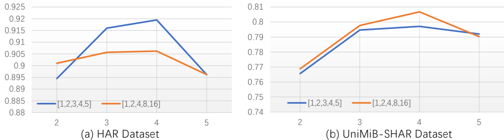
Figure 2: Multi-scale sampling strategies analysis under Sym 50% noisy labels.
