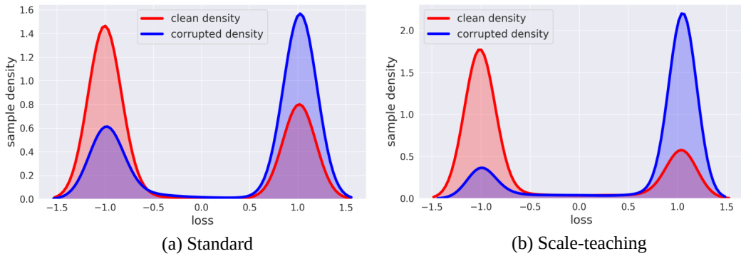
Figure 6: The loss value probability distributions visualization on UniMiB-SHAR dataset with Asym 40% noisy labels.
