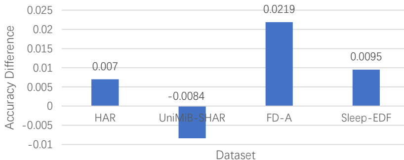
Figure 3: The cross fusion direction of input scale series analysis under Sym 50% noisy labels.
