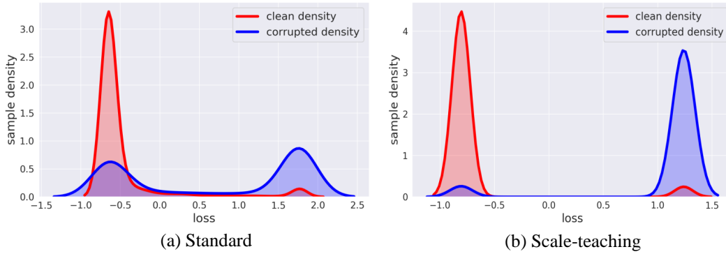
Figure 5: The loss value probability distributions visualization on HAR dataset with Asym 40% noisy labels.
