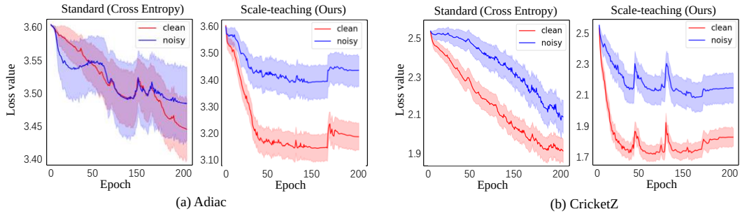
Figure 4: The change of loss values for clean and noisy time series samples under Asym 40% noise labels. The solid line and shading indicate the mean and standard deviation loss values of all clean (or noisy) training samples within each epoch.
