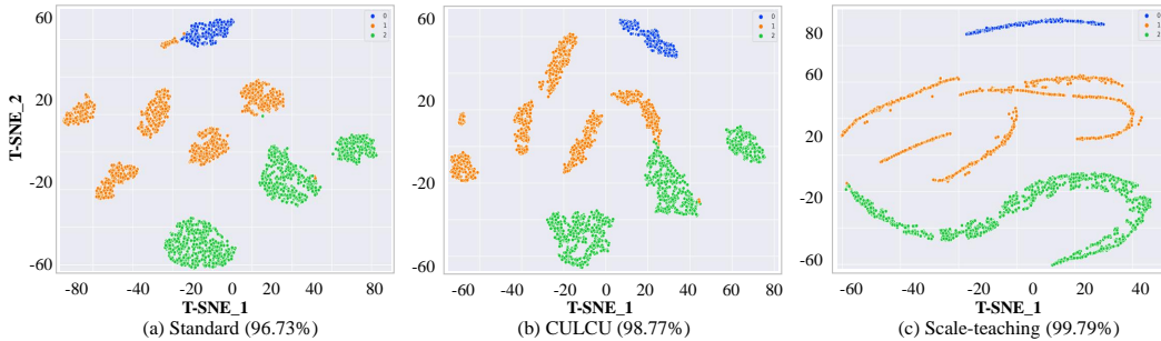
Figure 1: t-SNE visualization of the learned embeddings on the FD-A dataset with Sym 50% noisy labels (values in parentheses are the test classification accuracies).
