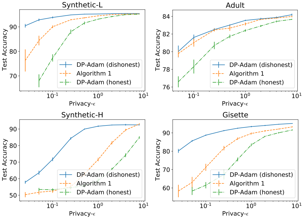
Figure 2: Comparison of Algorithm 1 against honest and dishonest DP-SGD baselines, varying \epsilon \in \{0.025, 0.05, 0.1, 0.25, 0.5, 1.0, 2.0, 4.0, 8.0\} and fixing \delta = 10^{-5} . On all three methods, we train the model for each learning rate on its grid (see Table 5) and report the test accuracy for the best learning rate on the grid. Results are averaged over 10 trials and the error bars on both sides of the mean values depict 1.96 times the standard error, giving the asymptotic 95% coverage.
