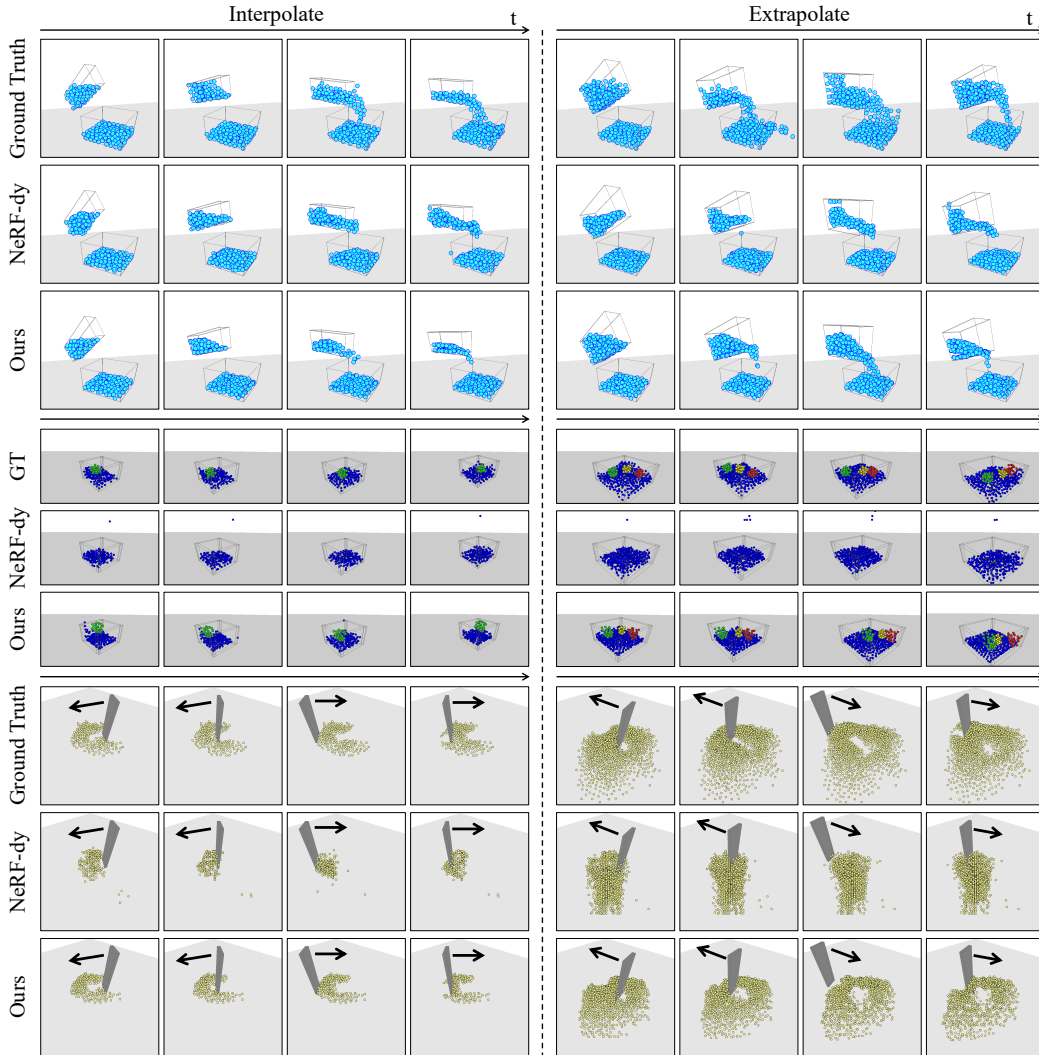
Figure 4: Qualitative Results of the Dynamics Module on Future Prediction. Here we visualize our model’s predicted future evolution of the particle set as compared with the NeRF-dy [34] baseline in both interpolate and extrapolate settings. Our method correctly identifies the shape/distribution of the fluids, rigid objects, and granular pieces with much better accuracy than NeRF-dy. The future evolution predicted by our method also matches the ground truth much better and produces reasonable results even in extrapolate settings.
