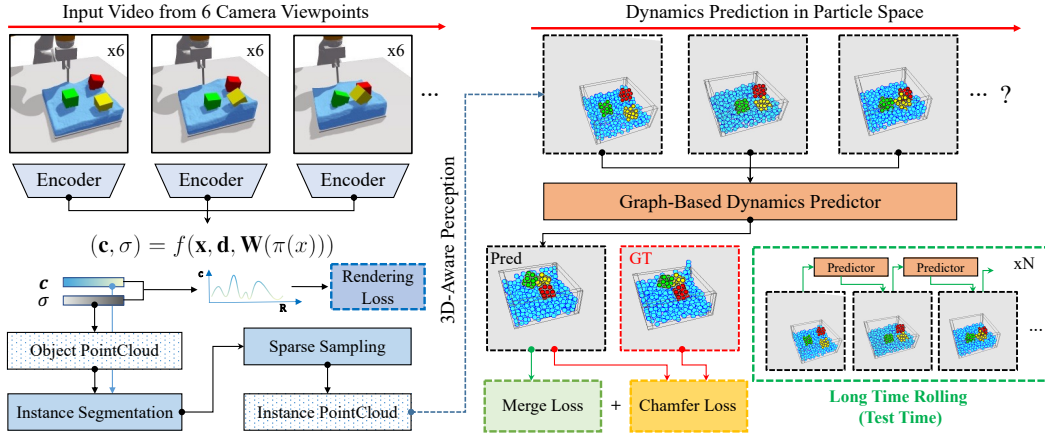
Figure 2: Overview of 3D Visual Intuitive Physics (3D-IntPhys). Our model consists of two major components: Left: The perception module maps the visual observations into implicit neural representations of the environment. We then subsample from the reconstructed implicit volume to obtain a particle representation of the environment. Right: The dynamics module, instantiated as graph neural networks, models the interaction within and between the objects and predicts the evolution of the particle set.
