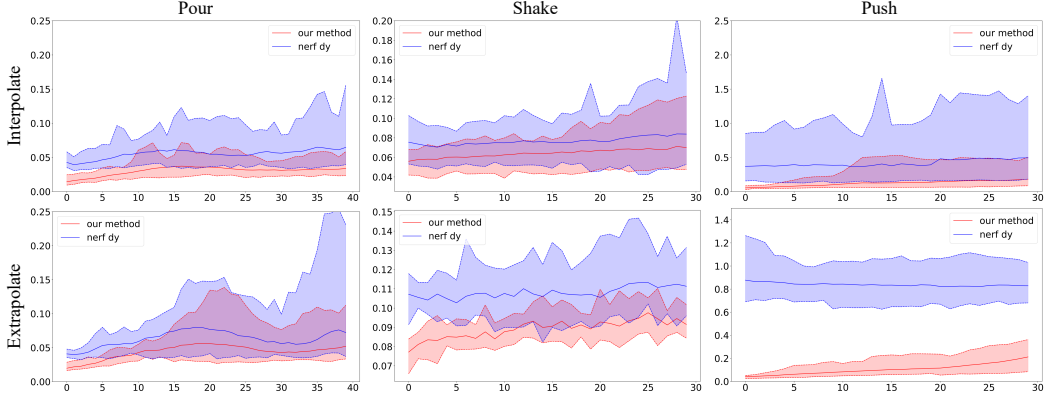
Figure 6: Quantitative Results of the Dynamics Module. This figure compares our method and NeRF-dy [34] on their long-horizon open-loop future prediction loss. The loss is measured as the Chamfer distance between the predicted particle set evolution and the actual future. Our method outperforms the baseline in both interpolate and extrapolate settings, showing the benefits of explicit 3D modeling.
