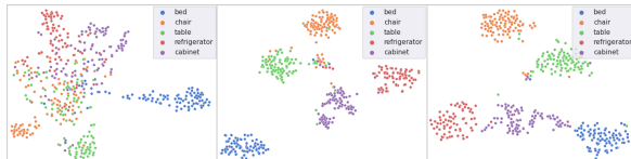
Figure 6: Visualize object-level embeddings with t-SNE.
