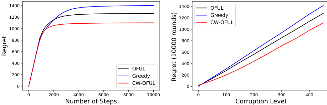
(a) Corruption level C = 450 . Cumulative regret versus Round
