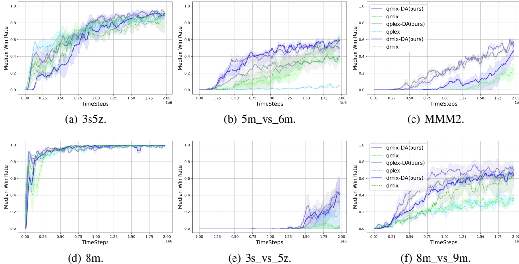
Figure 4: Results of QMIX, QPLEX and DMIX with or without integrated DAgger in six environments, showing that integrated DAgger can significantly increase the median win rate in 0 sight view.
