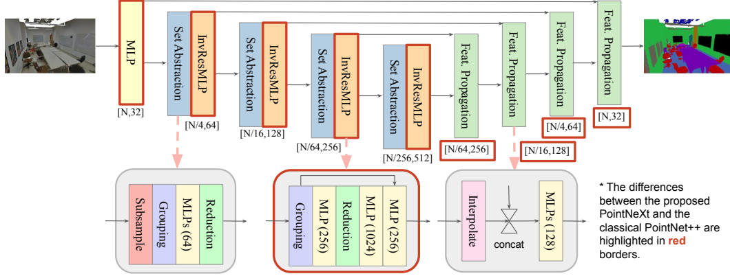
Figure 2: PointNeXt architecture. PointNeXt shares the same Set Abstraction and Feature Propagation blocks as PointNet++ [28], while adding an additional MLP layer at the beginning and scaling the architecture with the proposed Inverted Residual MLP (InvResMLP) blocks.
