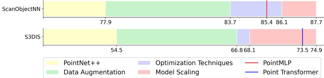
Figure 1: Effects of training strategies and model scaling on PointNet++ [28]. We show that improved training strategies (data augmentation and optimization techniques) and model scaling can significantly boost PointNet++ performance. The average overall accuracy and mIoU (6-fold cross-validation) are reported on ScanObjectNN [42] and S3DIS [1].
