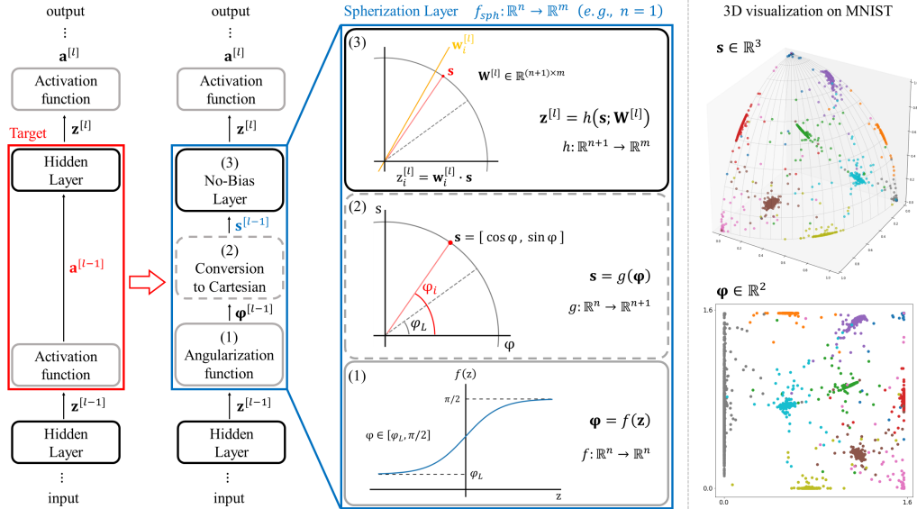
Figure 1: Overview of spherization layer . The red box indicates the existing fully connected layer to be replaced with the spherization layer in the blue box. After replacement, the pre-activations from (l - 1) th layer are passed to the angularization function, not activation function. These pre-activations are converted to angular coordinates in (1). Through (2), spherized representations are located on the (n + 1) -spherical surface. Finally, a hidden layer without bias parameters is trained on these spherized representations for using only the angles in (3). These relations of the input and output of the stage (1), (2), and (3) are illustrated as graphs, which are clearly defined in Eq. 3, Eq. 6, and Eq. 9, respectively. The right side displays how to generate angular coordinates and convert them to Cartesian coordinates in a 3-dimensional space on MNIST
