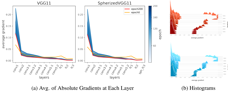
Figure 4: Analysis of Gradient Flow from Image Classification Model trained on CIFAR100. (a) The y-axis means the average of absolute gradients which occurred at each layer. The left side shows the gradient flow in VGG-11 (VGG11), and the right side shows the spherized VGG-11 (SpherizedVGG11), where the last fully connected layer is substituted with the spherization layer. (b) The histograms show the frequency of the average of absolute gradients in VGG-11 (red) and the spherized VGG-11 (cyan), respectively.
