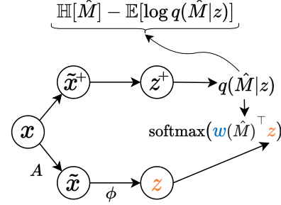
Figure 6: DISSL. The teacher (top branch) is trained with the top loss to ensure \hat{M} is a maximal invariant r.v. The student (bottom branch) distills the teacher by predicting \hat{M} .
