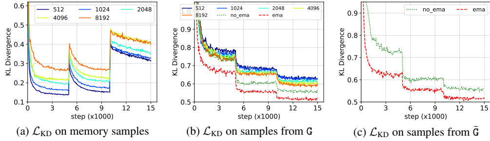
Figure 3: Distillation loss curves on memory samples (a) and samples generated by G (b) and \tilde{G} (c). The numbers in the legends denote DFKD-Mem with the corresponding memory sizes. “no_ema” and “ema” denote ABM and MAD, respectively.
