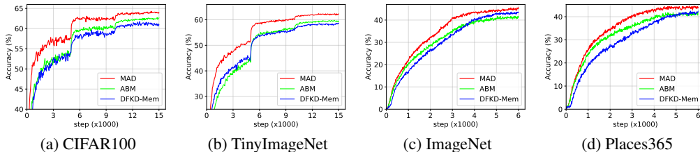
Figure 2: Test accuracy curves of S trained via MAD, ABM, and DFKD-Mem on some datasets.
