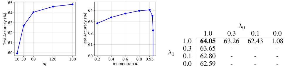
Figure 6: Test accuracy of our method w.r.t. different values of student update steps n_s (left), of the momentum \alpha (middle), and of the coefficients ( \lambda_0, \lambda_1 ) in Eq. 4 (right). The dataset is CIFAR100.
