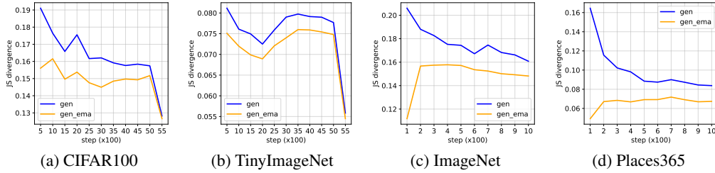
Figure 4: Average Jensen-Shannon divergences between the prediction probabilities of S_{t-\tau} and T computed on synthetic samples from G_t (labeled as “gen”) and \tilde{G}_t (labeled as “gen_ema”) for different datasets. For CIFAR100 and TinyImageNet, we set t \in [500, 5500] with step size of 500 and \tau = 50 . For ImageNet and Places365, we set t \in [100, 1000] with step size of 100 and \tau = 10 . Note that the sudden drops at step 5000 in (a), (b) correspond to the decay of the learning rate by 0.1.
