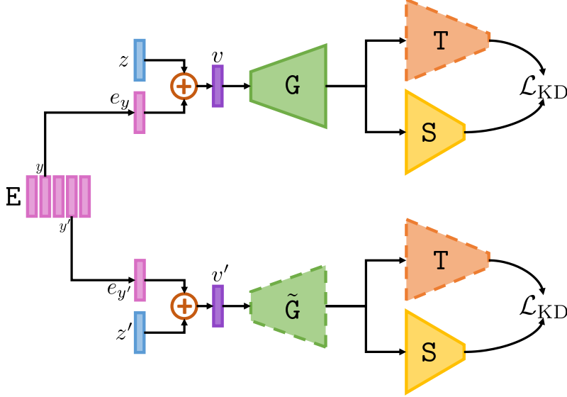
Figure 1: An illustration of our proposed Momentum Adversarial Distillation (MAD) consisting of a teacher (T), a student (S), a class-conditional generator (G), an EMA generator ( \tilde{G} ), and class embeddings (E). Networks with dashed borders (T, \tilde{G} ) are not optimized during training. z and z' are random noises sampled from \mathcal{N}(0, I) . e_y and e_{y'} are gathered from E at index y and y' , respectively.
