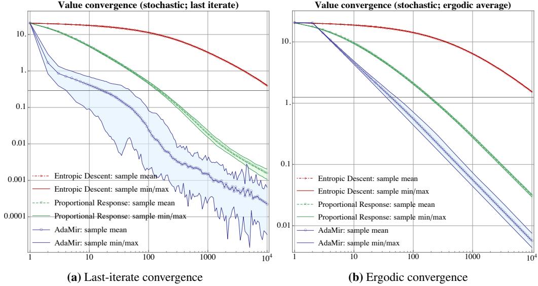
Figure 4: Statistics for the convergence speed of (EGD), (PR) and ADAMIR in a stochastic Fisher market, with marginal utilities drawn i.i.d. at each epoch. The marked lines are the observed means from S = 50 realizations, whereas the shaded areas represent a 95% confidence interval.
