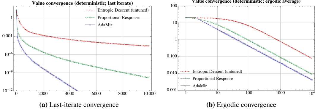
Figure 2: The convergence speed of (EGD), (PR) and ADAMIR in a stationary Fisher market.
