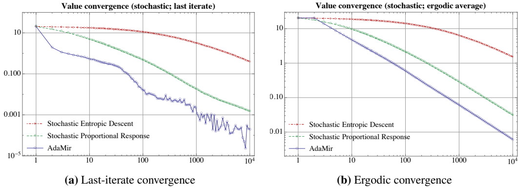
Figure 3: The convergence speed of (EGD), (PR) and ADAMIR in a stochastic Fisher market, with marginal utilities drawn i.i.d. at each epoch.
