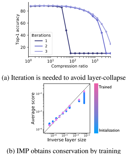
Figure 5: How IMP avoids layer collapse. (a) Multiple iterations of training-pruning cycles is needed to prevent IMP from suffering layer-collapse. (b) The average square magnitude scores per layer, originally at initialization (blue), converge through training towards a linear relationship with the inverse layer size after training (pink), suggesting layer-wise conservation. All data is from a VGG-19 model trained on CIFAR-10.
