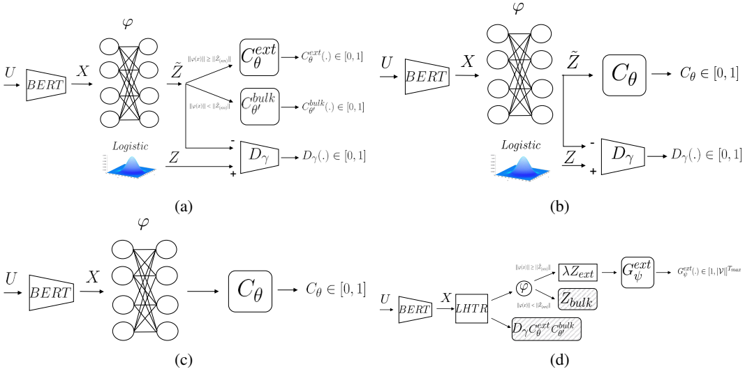
Figure 4: Illustrative pipelines.
