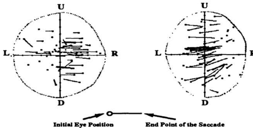
Figure 1: Eye Movements Evoked by Electrical Stimulations in V1
