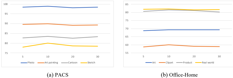
Figure 1: Impact of the epoch of warm-up stage on (a) PACS and (b) Office-Home using ResNet-50 as the backbone. Note that x and y axes denote the epoch of warm-up stage and top-1 classification accuracy (%), respectively.
