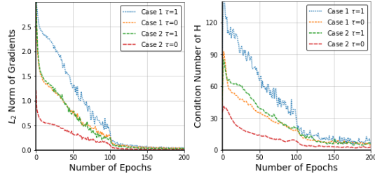
Figure 4: The condition number of H_t and the \ell_2 norm of full gradient (i.e., \| \nabla f(x_t) \|_2 ) for CIFAR-10 by our SUPER-ADAM algorithm \tau = 1 and \tau = 0 , respectively. Cases 1 and 2 are two choices of adaptive matrix H_t given in Algorithm 1.
