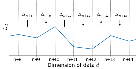
Figure 2: Illustration of the multiple descent phenomenon for the generalization loss L_d versus the dimension of data d in the overparametrized regime starting from d = n + 8 . One can fully control the generalization curve to increase or decrease as specified by the sequence \Delta = \{\downarrow, \uparrow, \downarrow, \downarrow, \uparrow, \downarrow, \dots\} . Adding a new feature with Gaussian mixture distribution increases the loss, while adding one with Gaussian distribution decreases the loss.
