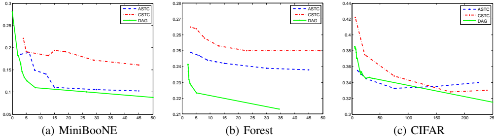
Figure 4: Comparison between CSTC, ASTC, and DAG of the average number of acquired features (x-axis) vs. test error (y-axis).
