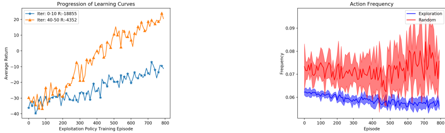
(a) Animat Results: Average learning curves on training tasks over the first 10 iterations (blue) and last 10 iterations (orange).
