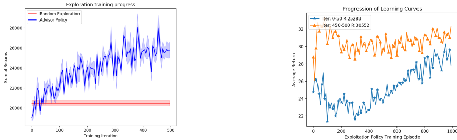
(a) Performance curves during training comparing advisor policy (blue) and random exploration policy (red).
