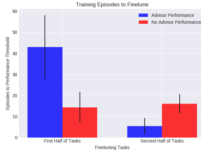
Figure 5: Number of episodes needed to achieve threshold performance (lower is better).
