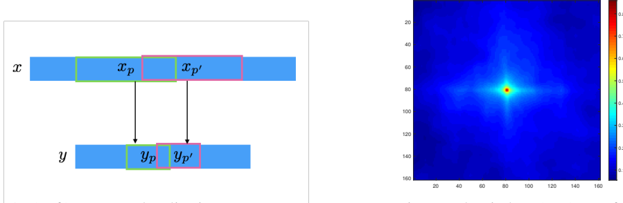
Figure 1: (Left) Between-locality in a sequence-to-sequence setting: each window (part) y_p of the output sequence y is fully determined by the part x_p of the input sequence x , for every p \in P . (Right) Empirical within-locality C_{p,q} of 100 images sampled from ImageNet between a 20 \times 20 patch q and the central patch p .
