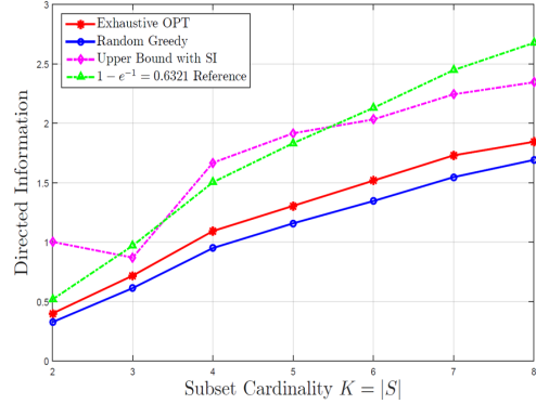
Figure 1: Solution and Bounds for OPT1 on D1 Figure 2: Solution and Bounds for OPT2 on ST
