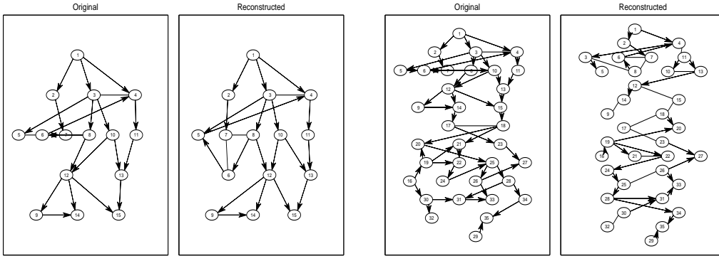
Figure 3: Ground truth structure (left) versus Reconstructed causal graph (right), D1 dataset
