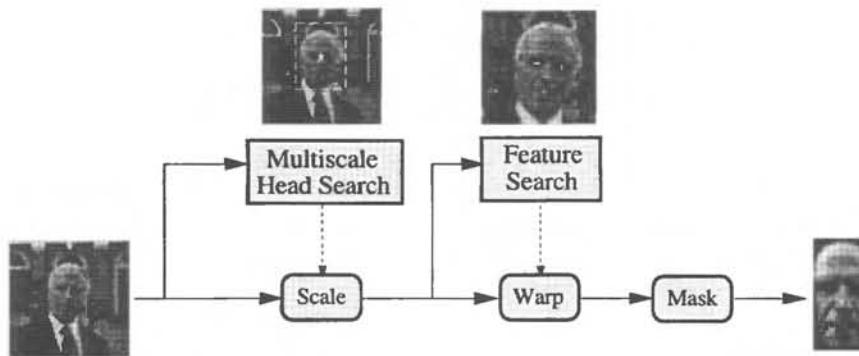
Figure 2: Face alignment system [7].
