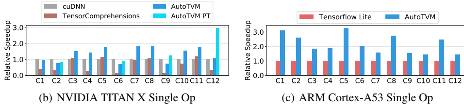
Figure 10: Single operator performance on the TITAN X and ARM CPU. (Additional ARM GPU (Mali) results are provided in the supplementary material.) We also included a weight pre-transformed Winograd kernel [24] for 3 \times 3 conv2d (AutoTVM PT). AutoTVM generated programs that were competitive with hardware-specific libraries.
